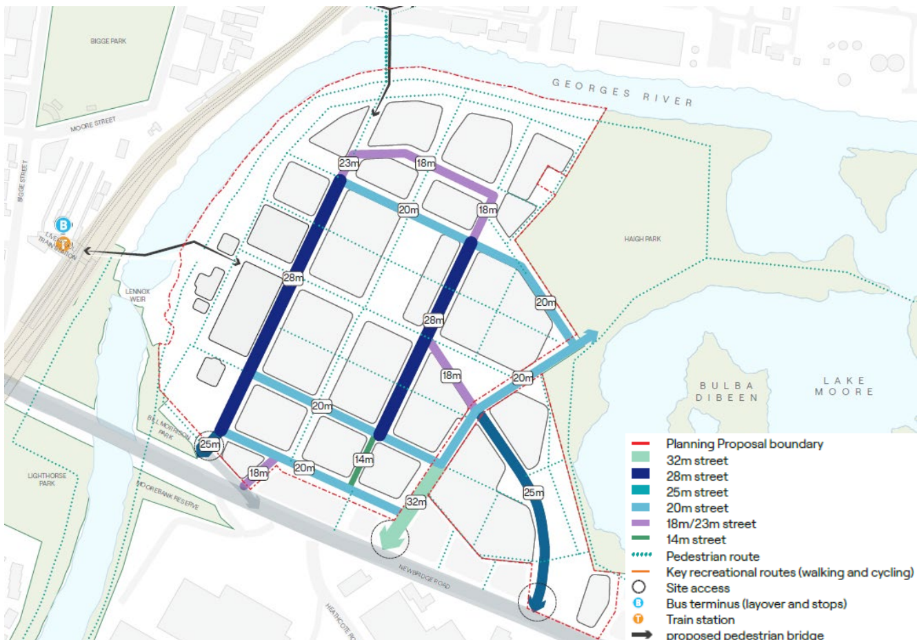
Figure 77: Street Hierarchy
