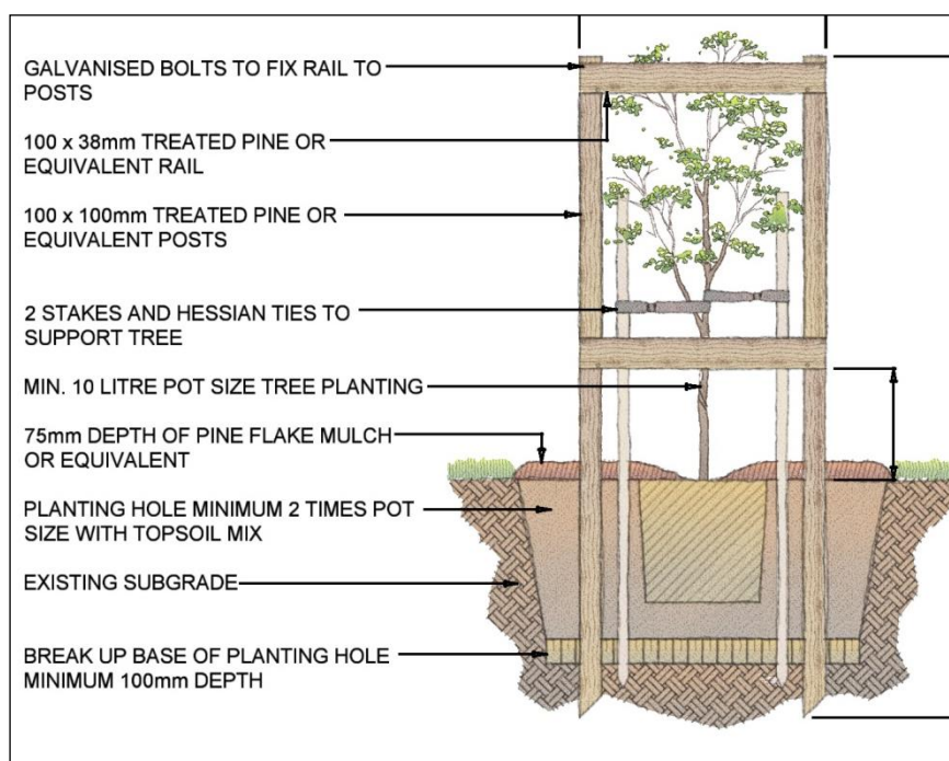
Figure 6 Tree Guard and Planting Details
