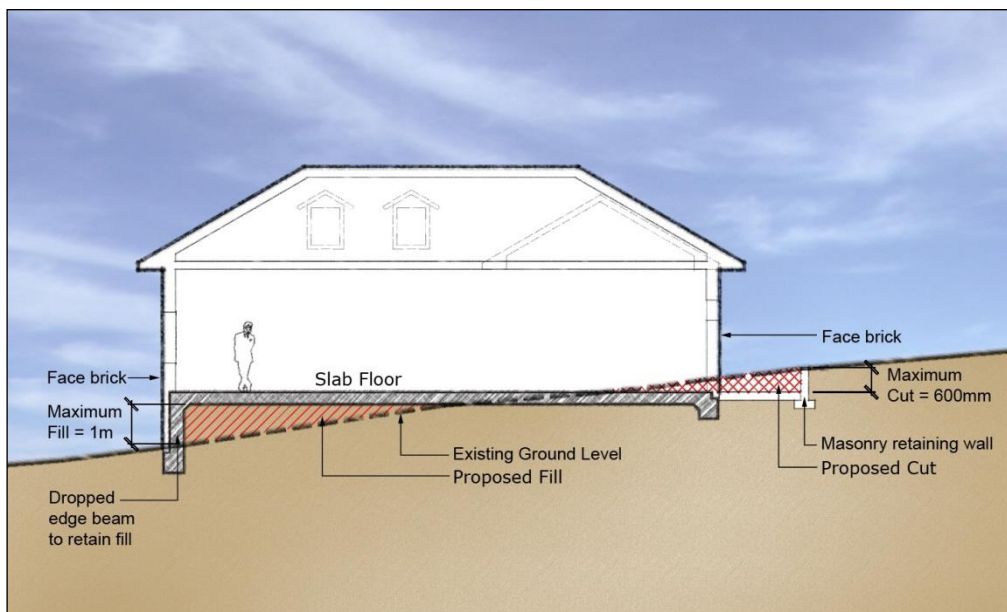
Figure 28 Cut and Fill requirements
