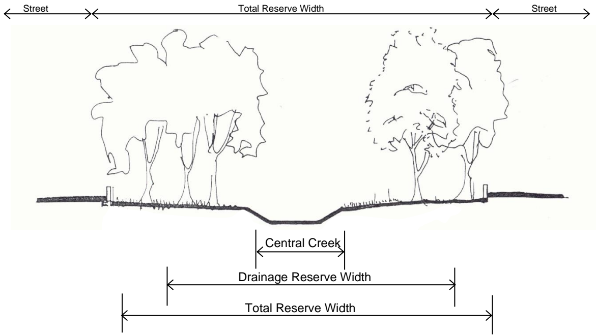
Figure 15 Type B Channel
