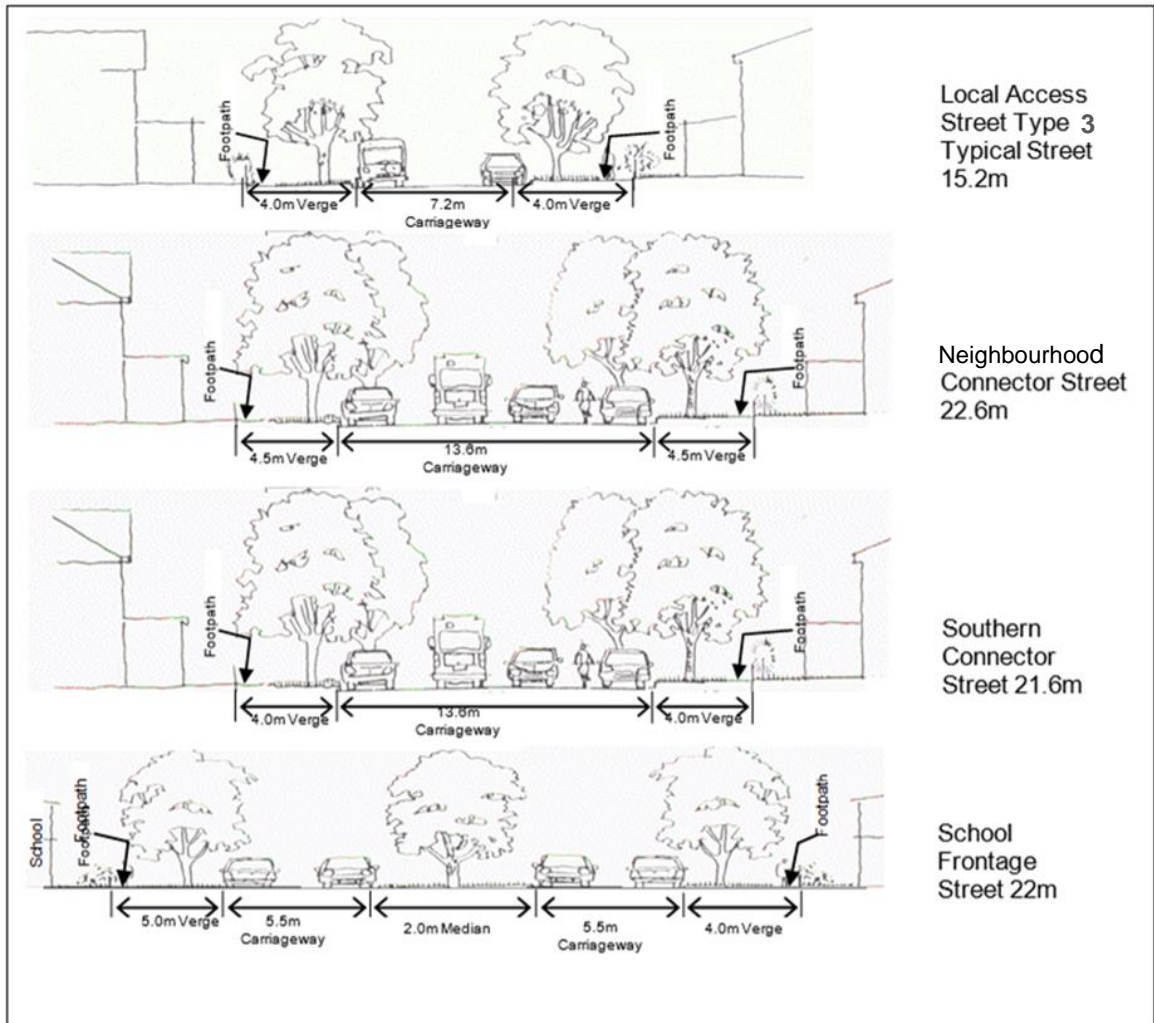
Figure 5 Street Sections
