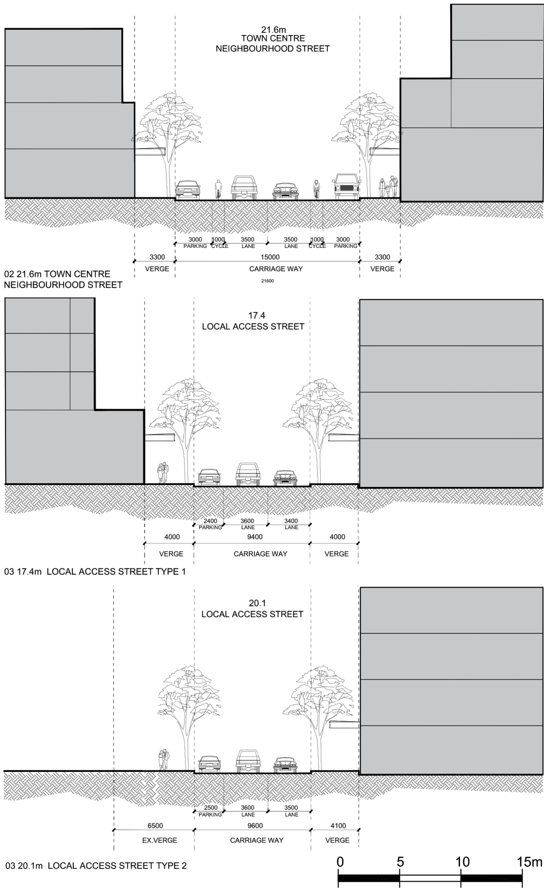
Figure 6 Local Centre Street Sections
