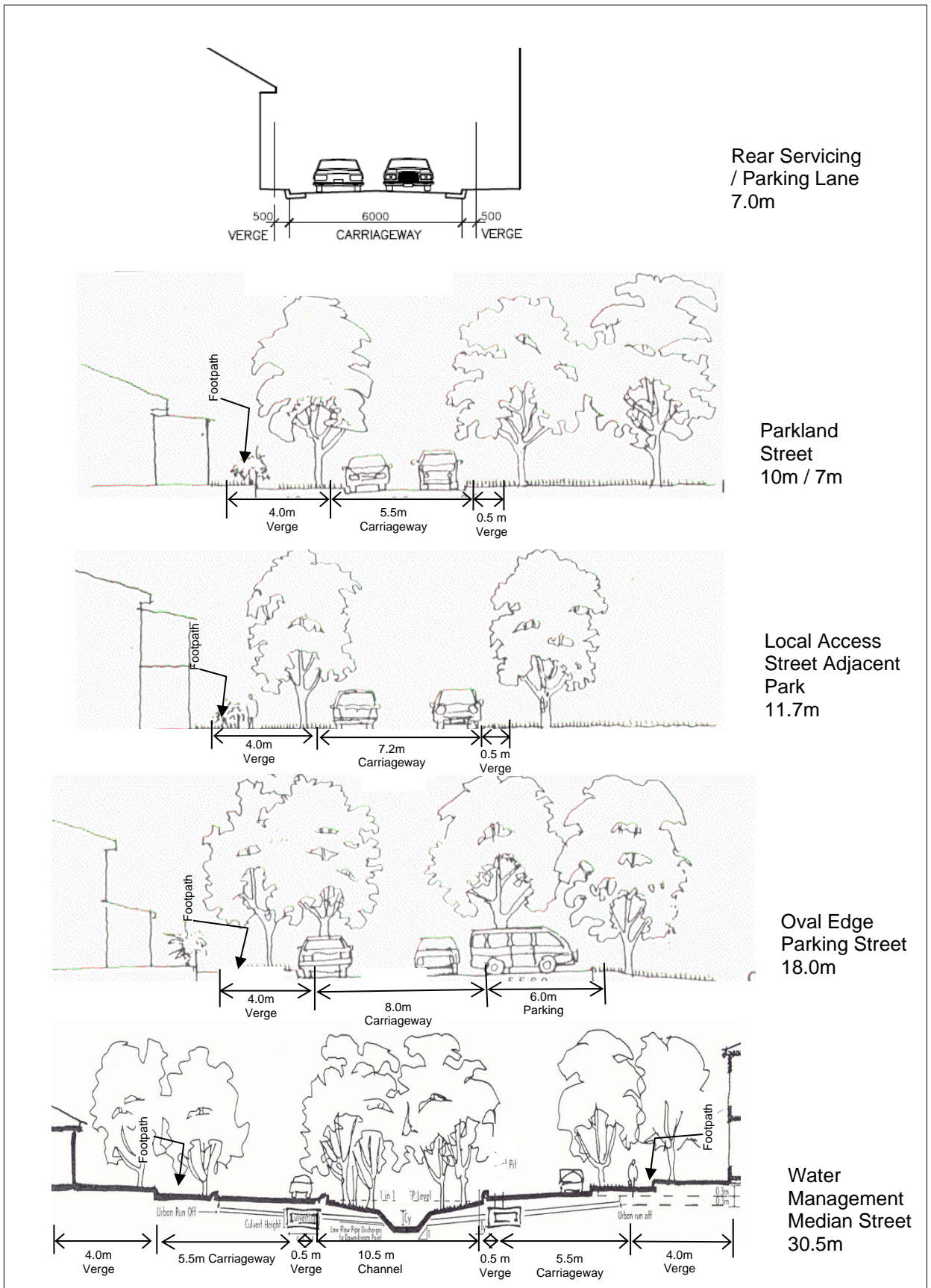
Figure 4 Street Sections
