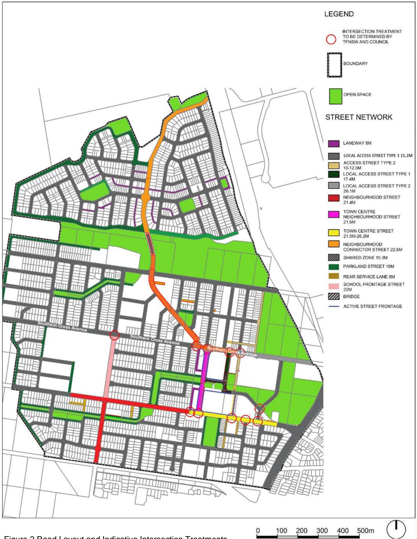
Figure 2 Road Layout and Indicative Intersection Treatments
