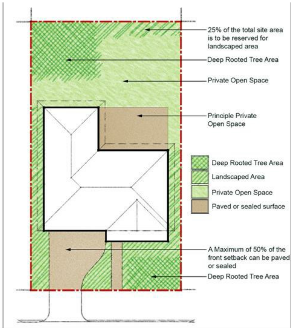
Figure 6 An example of Landscaped Area and Private Open Space
