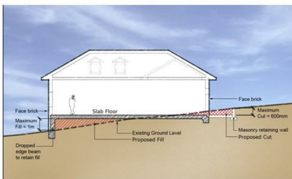
Figure 7 Example of Cut and Fill
