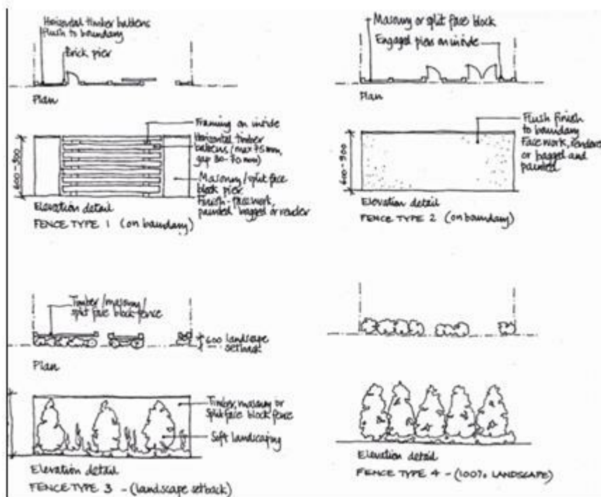
Figure 16 Fence Principles in plan
