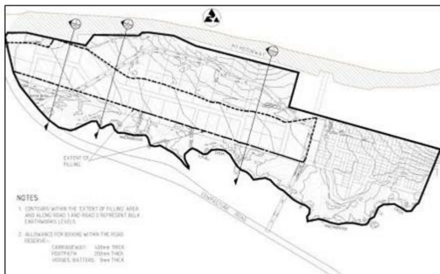
Figure 9 Areas of Site Fill
