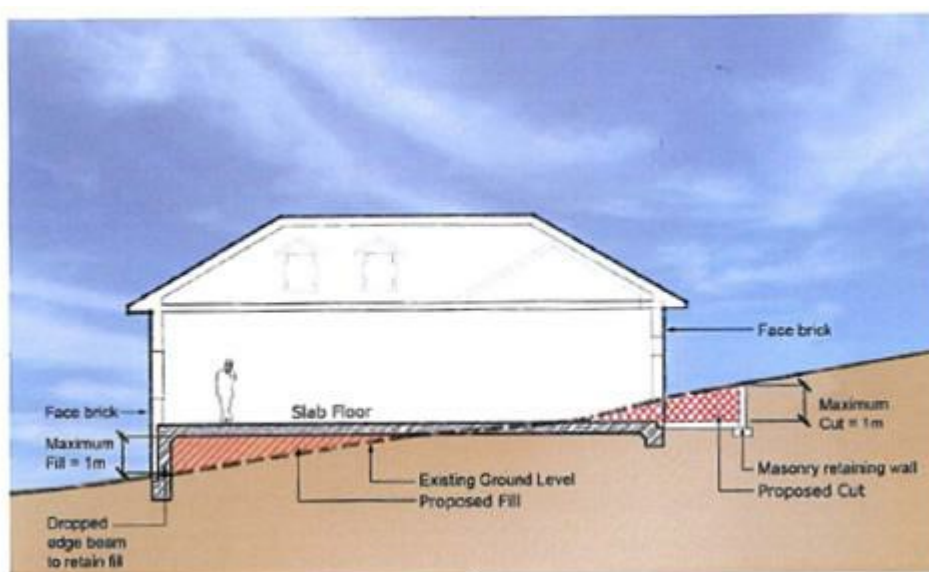
Figure 17: Cut & Fill Requirements
