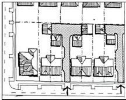
Figure 21: Private Driveways
