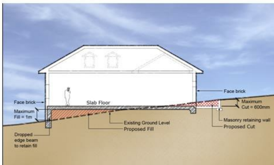
Figure 44: An example of Cut and Fill
