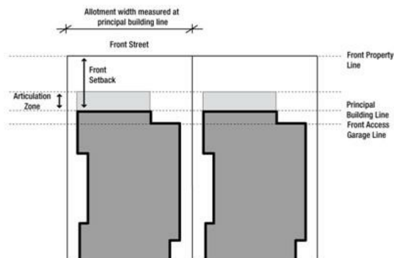
Figure 28: Front Setback Line
