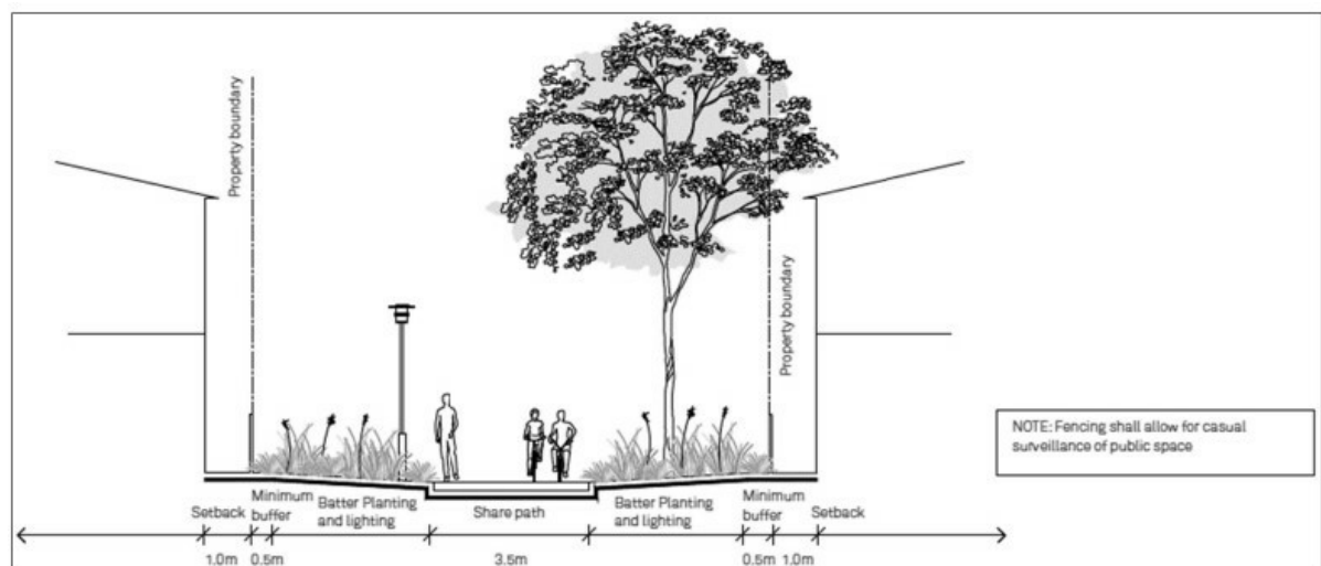
Figure 18: Pedestrian Access Way
