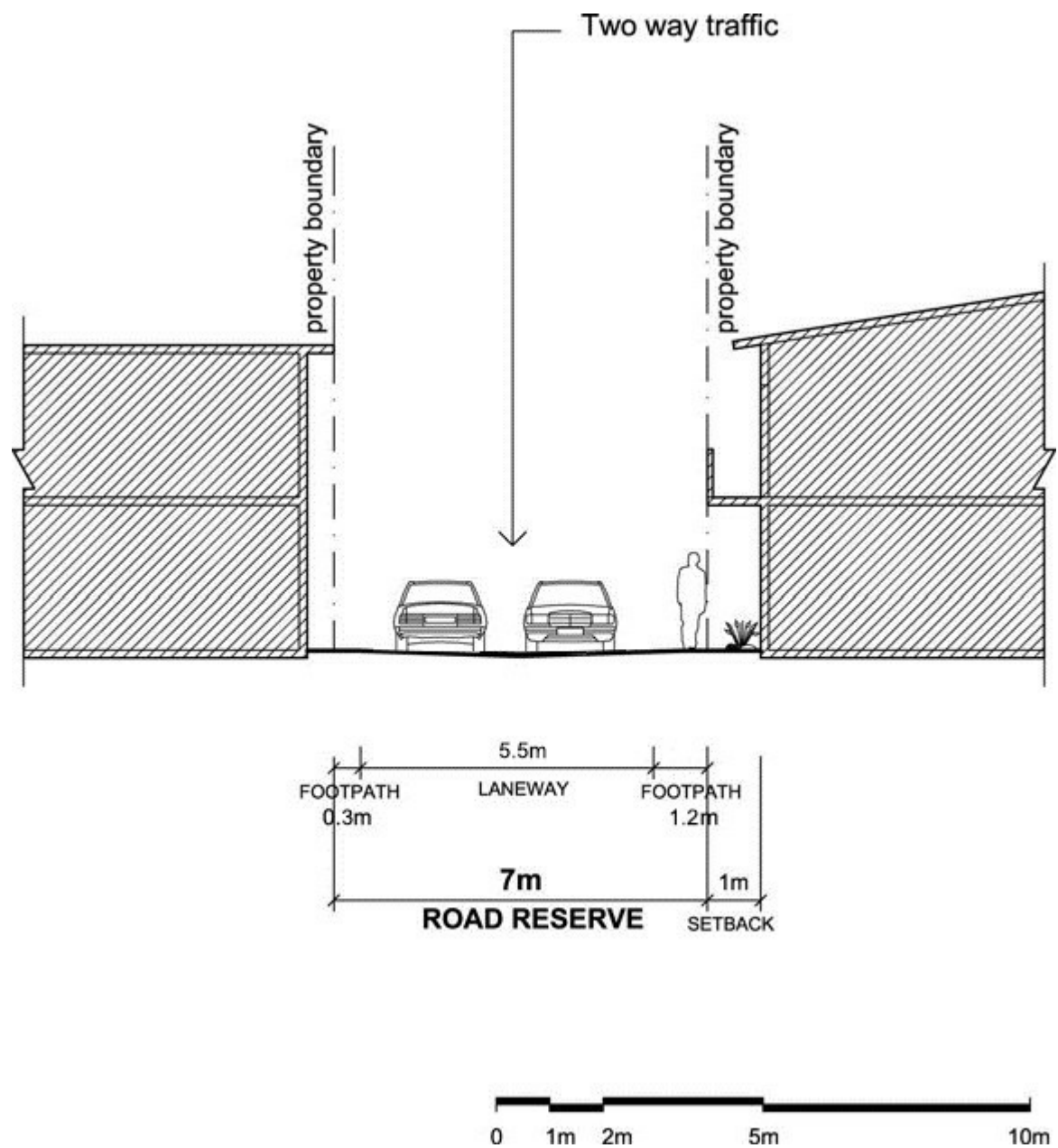
Figure 16 Residential Laneway
