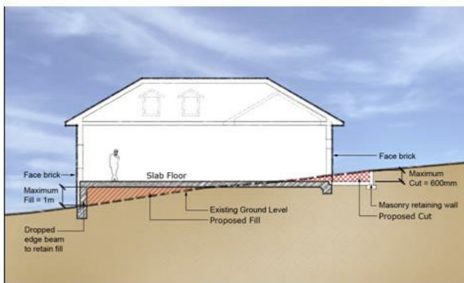
Figure 39: An example of Cut and Fill
