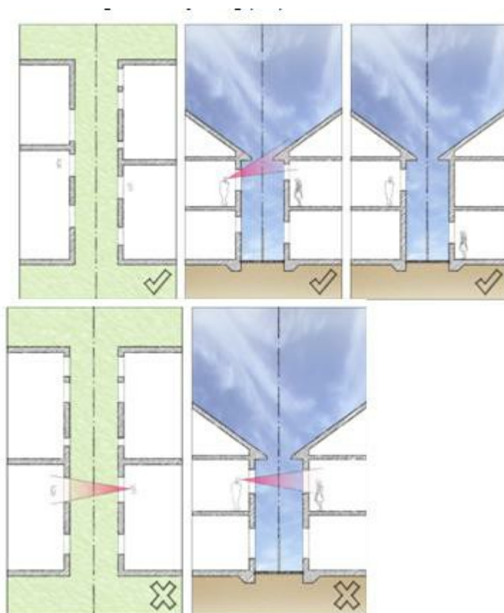
Figure 8 Plan views of windows being offset
