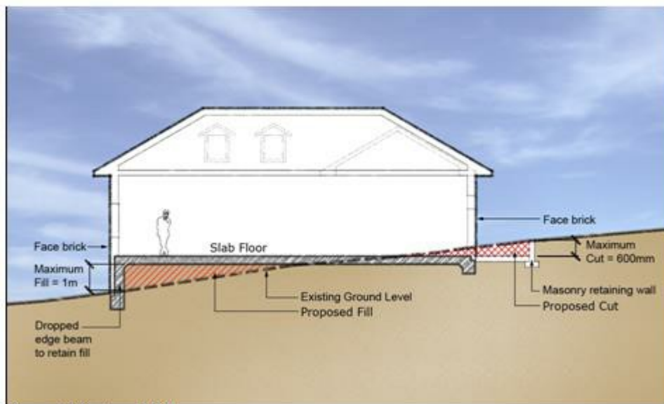
Figure 6 Cut and Fill
