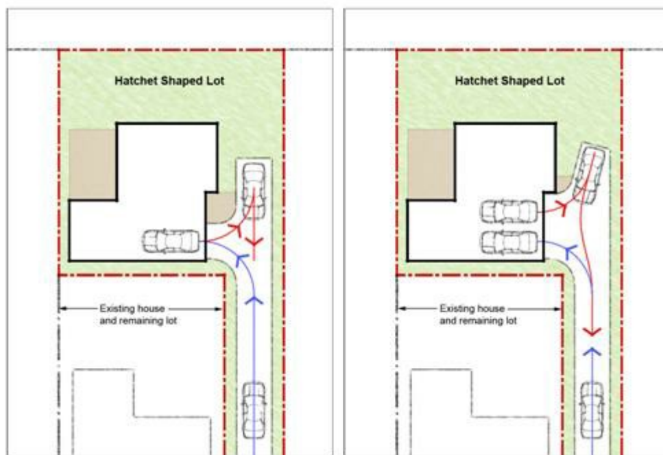
Figure 3 Driveway Layout and access
