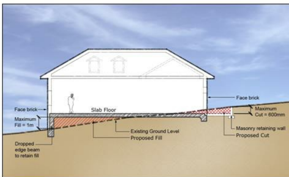
Figure 5 Cut and Fill
