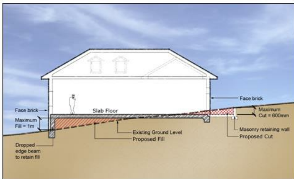
Figure 15 Cut and Fill requirements for a dwelling
