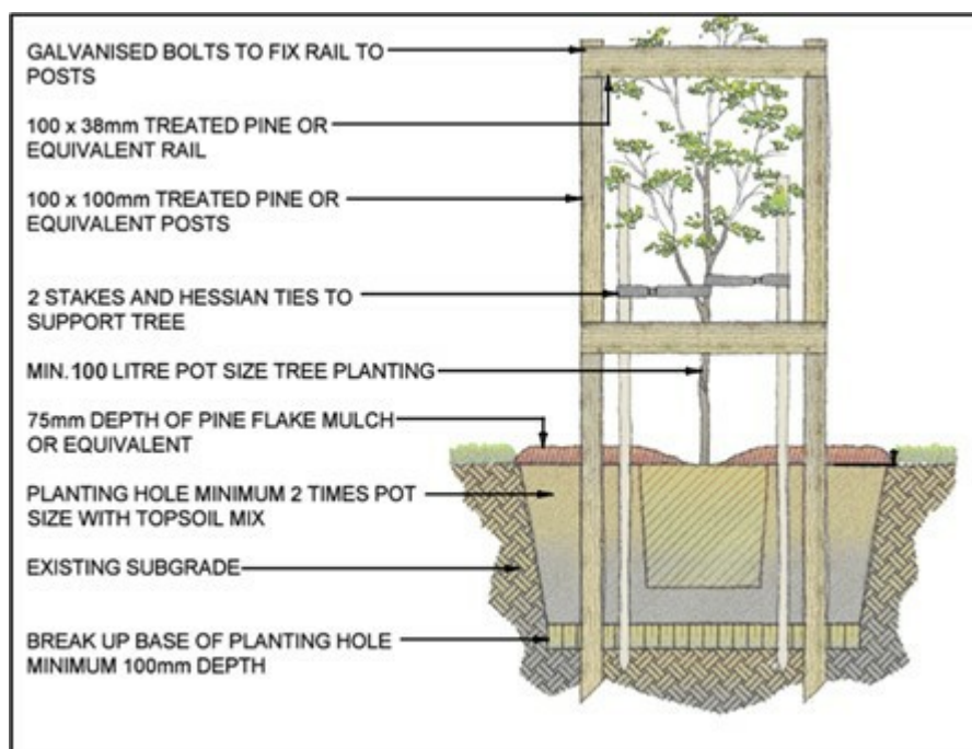
Figure 6 Tree Protection and Planting Details
