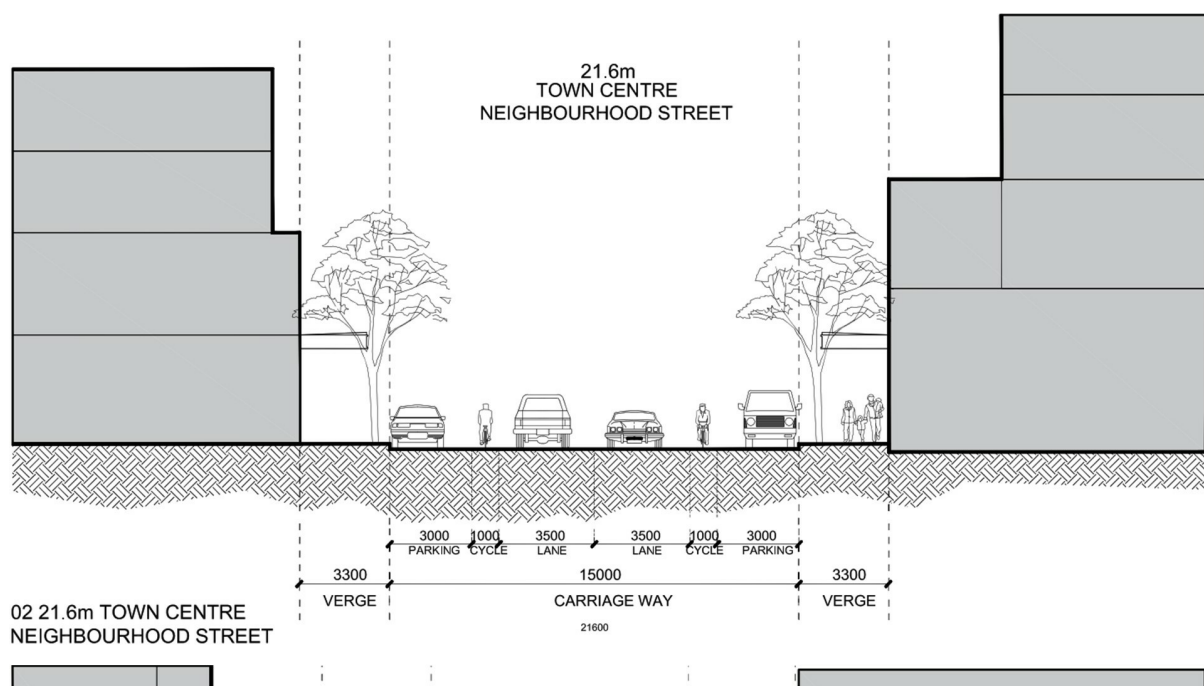
Figure 5 Street Sections
