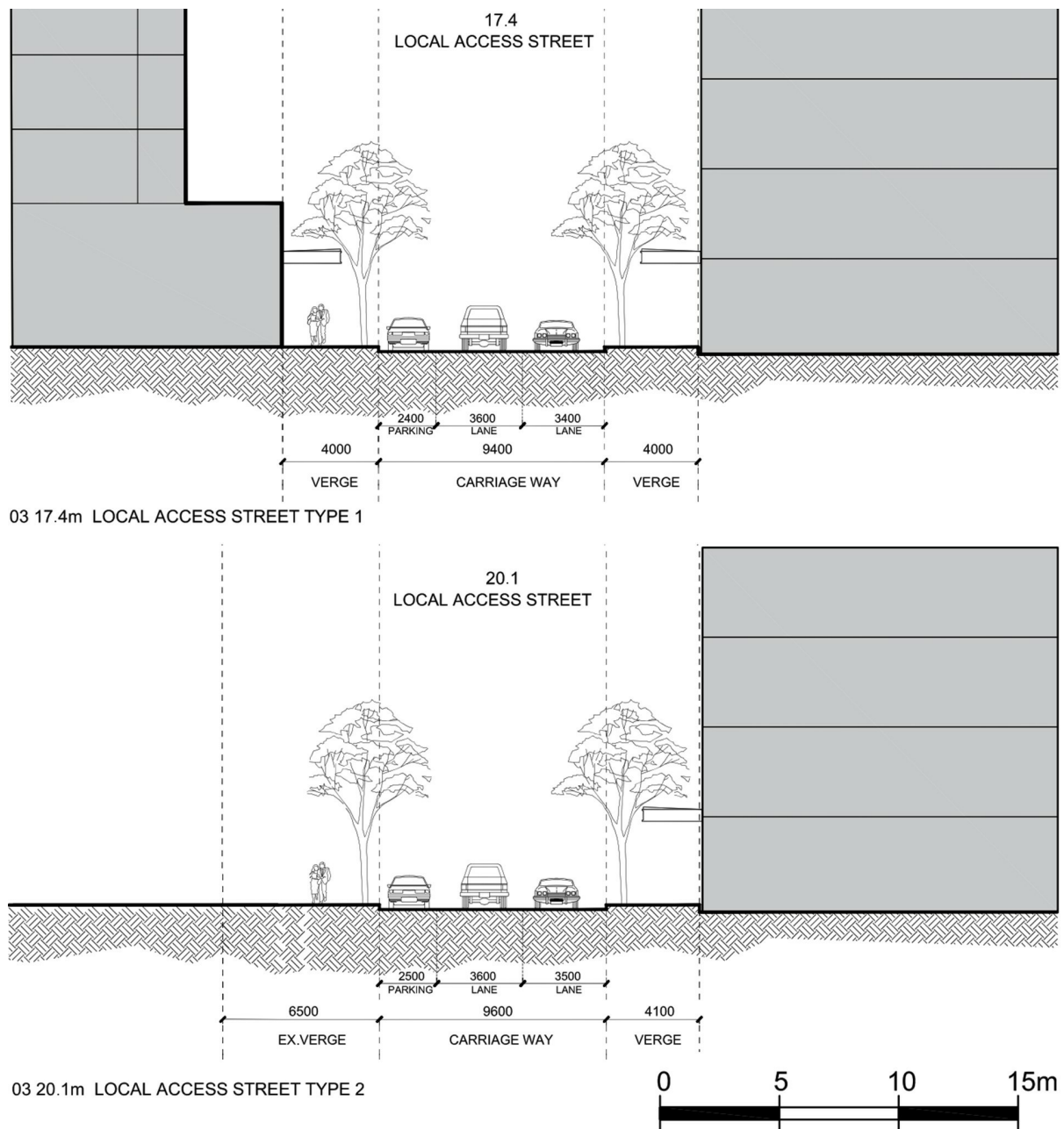
Figure 6 Local Centre Street Sections
