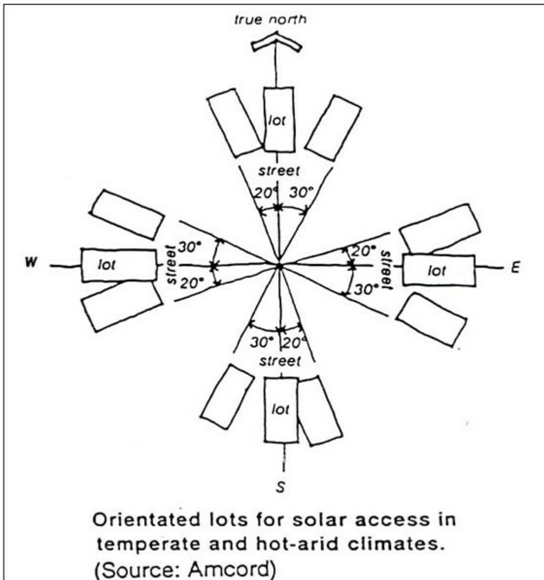
Figure 22 Lot Orientation
