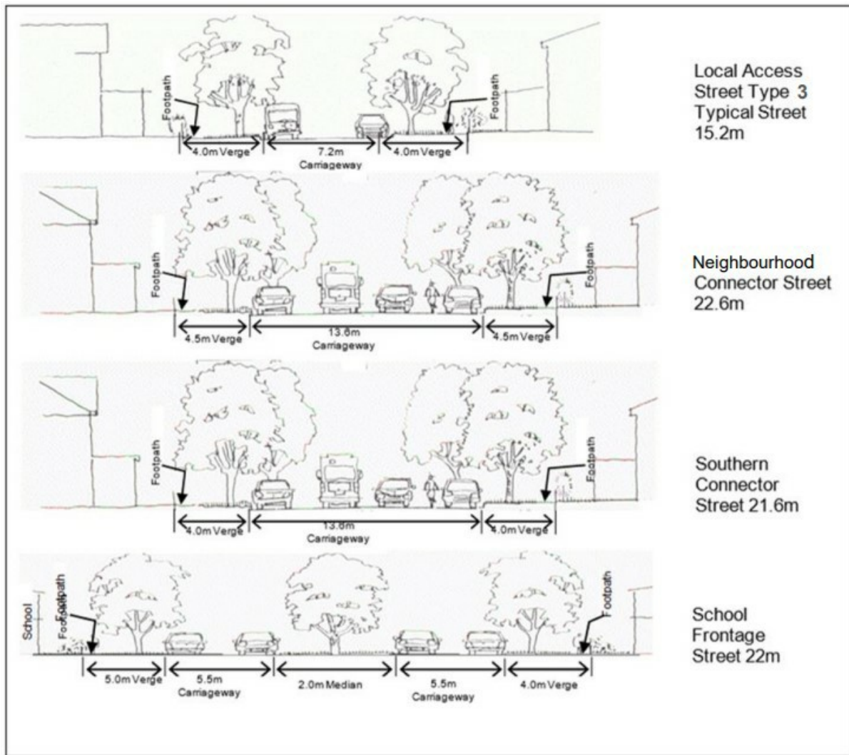
Figure 5 Street Sections
