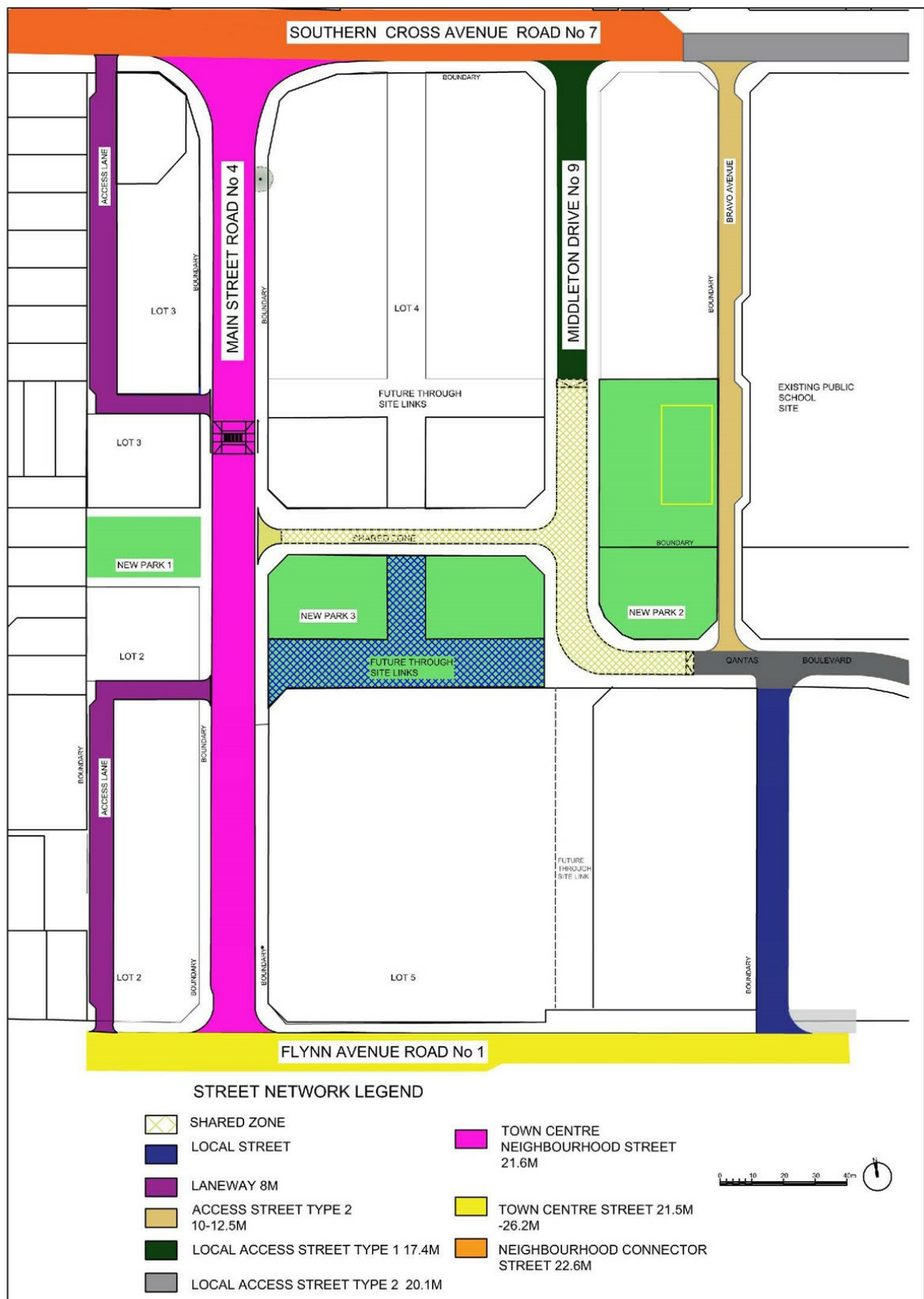
Figure 3 Local Centre Street Design
