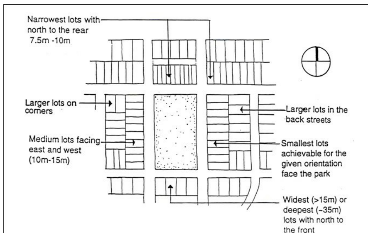
Figure 21 Lot Orientation
