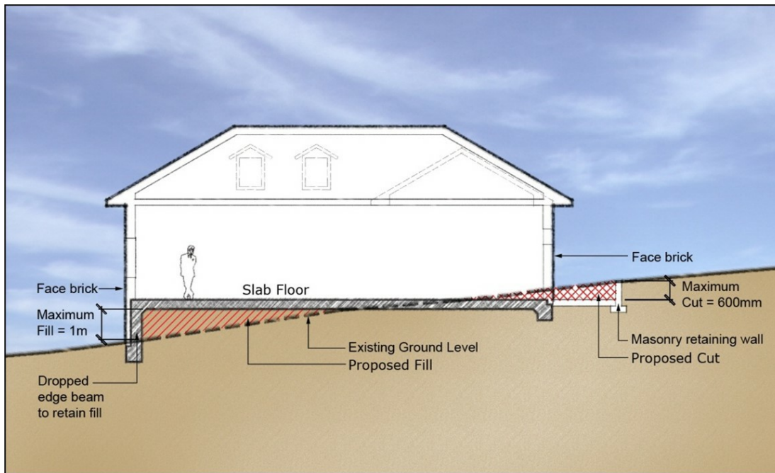
Figure 28 Cut and Fill requirements
