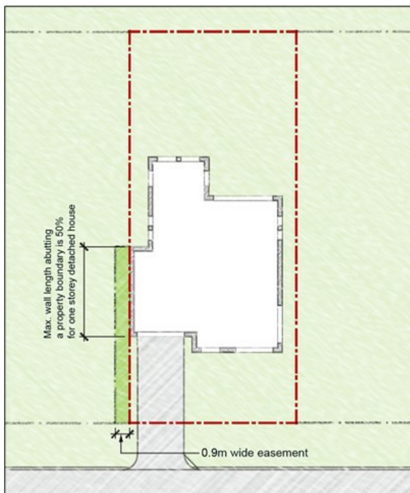
Figure 25 Zero Lot Lines
