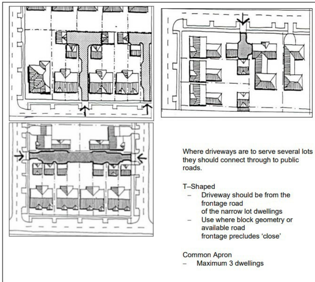
Figure 31 Private Driveways
