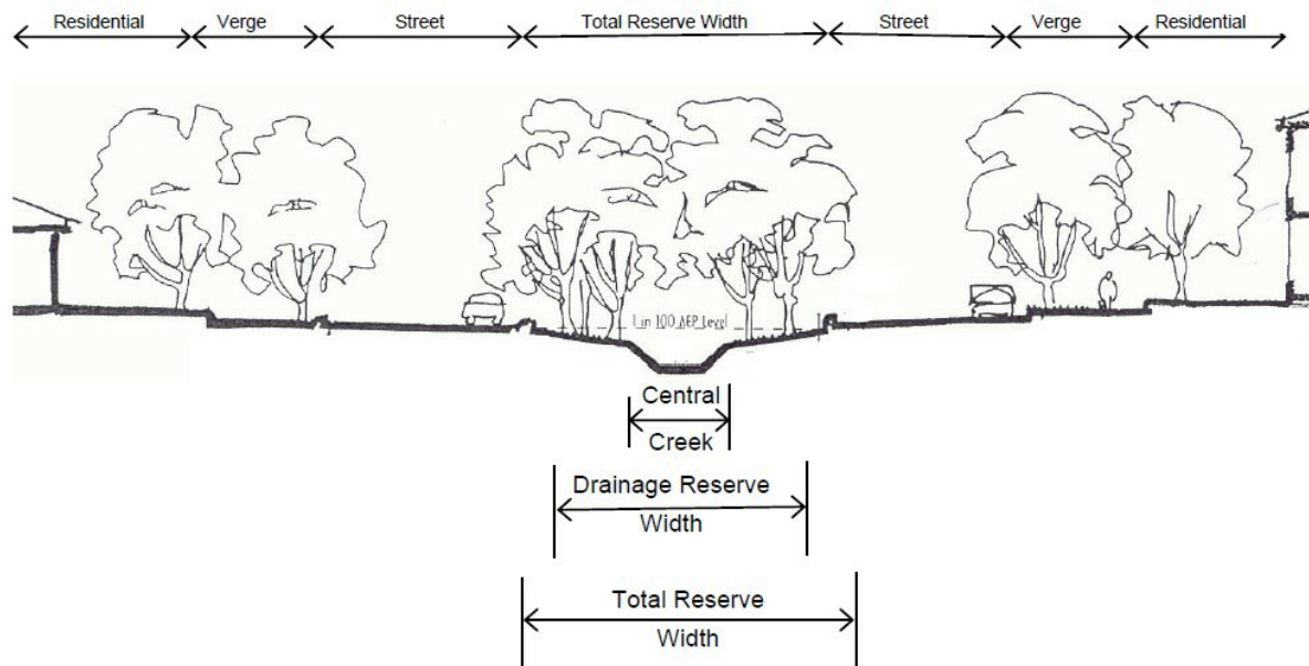
Figure 14 Type A Channel
