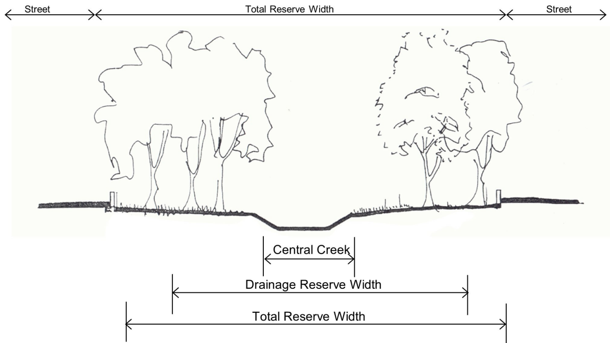
Figure 15 Type B Channel
