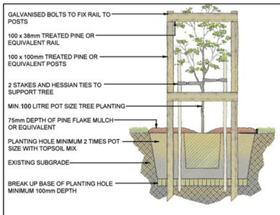
Figure 12 Tree Protection
