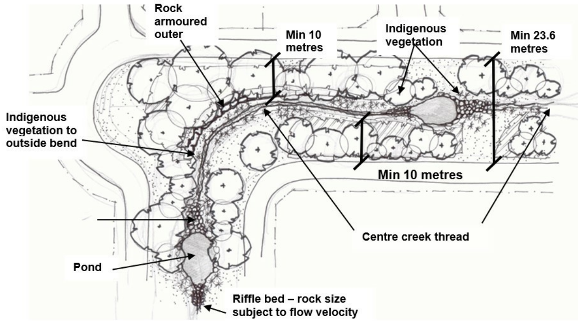
Figure 19 Creek Corridor
