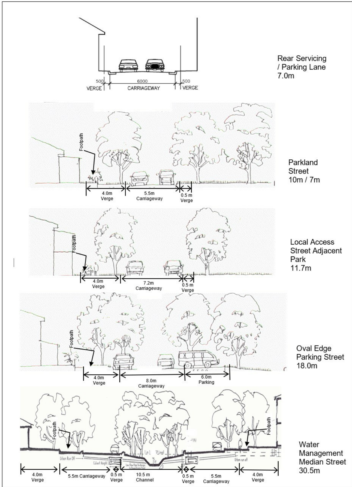
Figure 4 Street Sections
