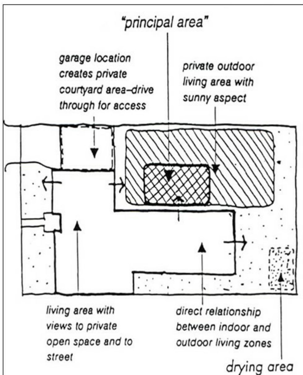
Figure 23 Private Open Space Considerations on an East-West Lot
