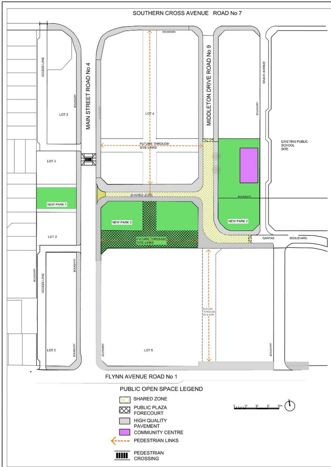
Figure 35 Local Centre Open Space
