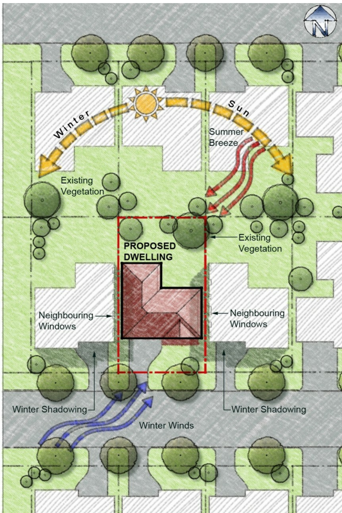
Figure 24 Example of a site analysis plan
